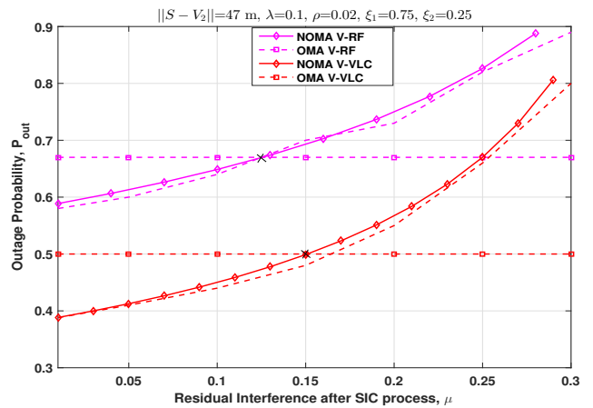
Fig. 9: Comparison of analytical (solid line) and simulation (dashed line) results for outage probability, P_{out} as a function of interference fraction left after SIC process for OPD NOMA based V-VLC link (red) and NOMA based V-RF link (magenta)
