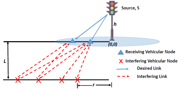
Fig. 3: Abstraction used for modelling. The desired vehicles are marked in triangle, while interferers are marked in cross marks. Here, L and h denotes the inter lane distance and height of traffic lamp respectively.
