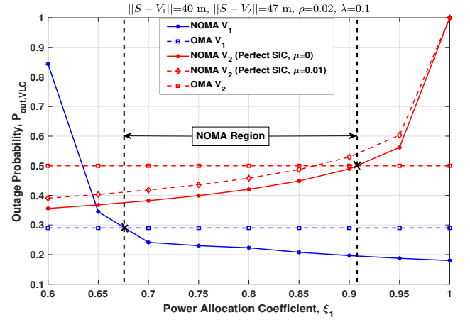
Fig. 6: Outage performance of V-VLC as a function of power allocation coefficient, \xi_1 for OMA (dashed) and NOMA (solid).
